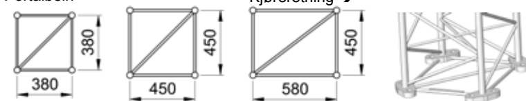
Portalbein
