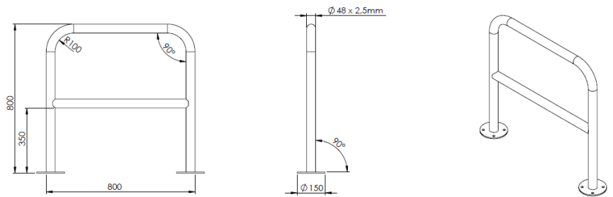
For overflatemontering
